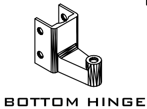
SPRING LOADED BOTTOM HINGE (INSIDE DOOR) RETURNS DOOR TO DESIRED OPEN POSITION WHEN NOT IN USE
