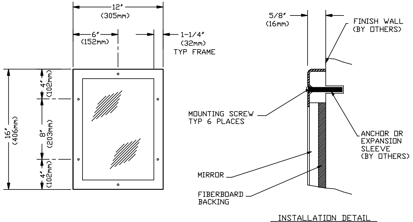
INSTALLATION DETAIL
