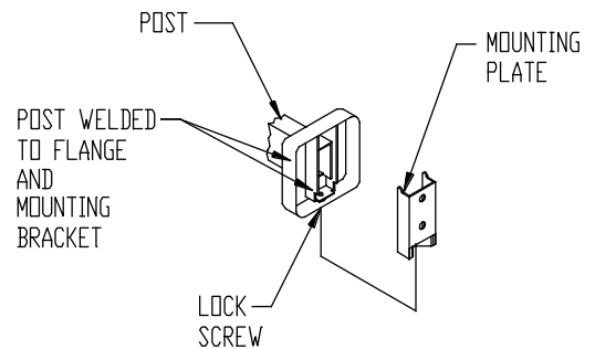
CONCEALED MOUNTING DETAIL
