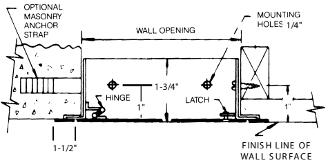
SECTION DETAIL
