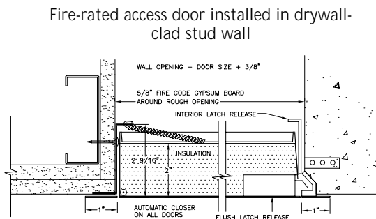
SECTION DETAIL
